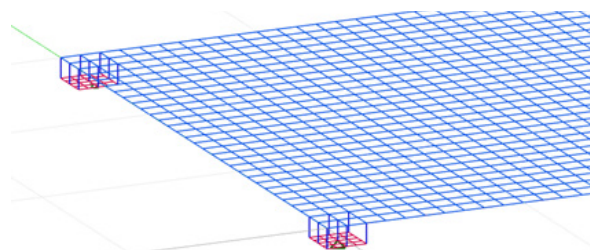
Figure 22: Modelling of point supports using additional elements
