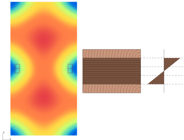
Figure 30: Largest bending stress in minor direction of rotated zones occurring in zones indicated by rectangles
