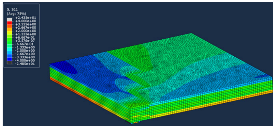
Figure 52: Stresses parallel to the grain
